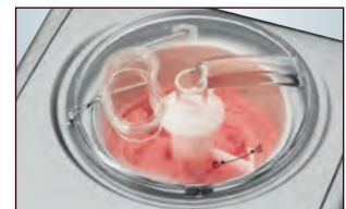
Transparent lid with refill opening
